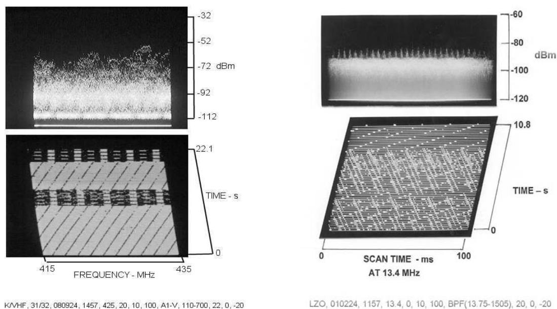
Figure 31 Severe Radio Interference from Variable-Speed Electric-Motor Drives
