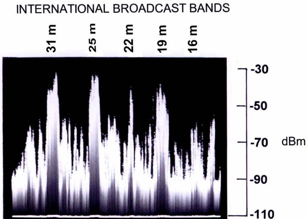
Figure 2 Example of Daytime Signal Levels in the HF Band
