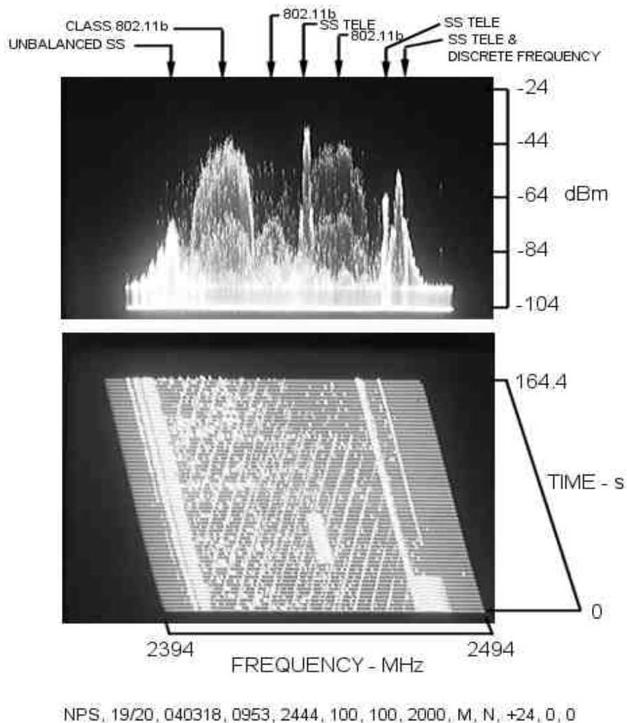
Figure 63 Example of Signals, Noise and Interference in the UHF Band
