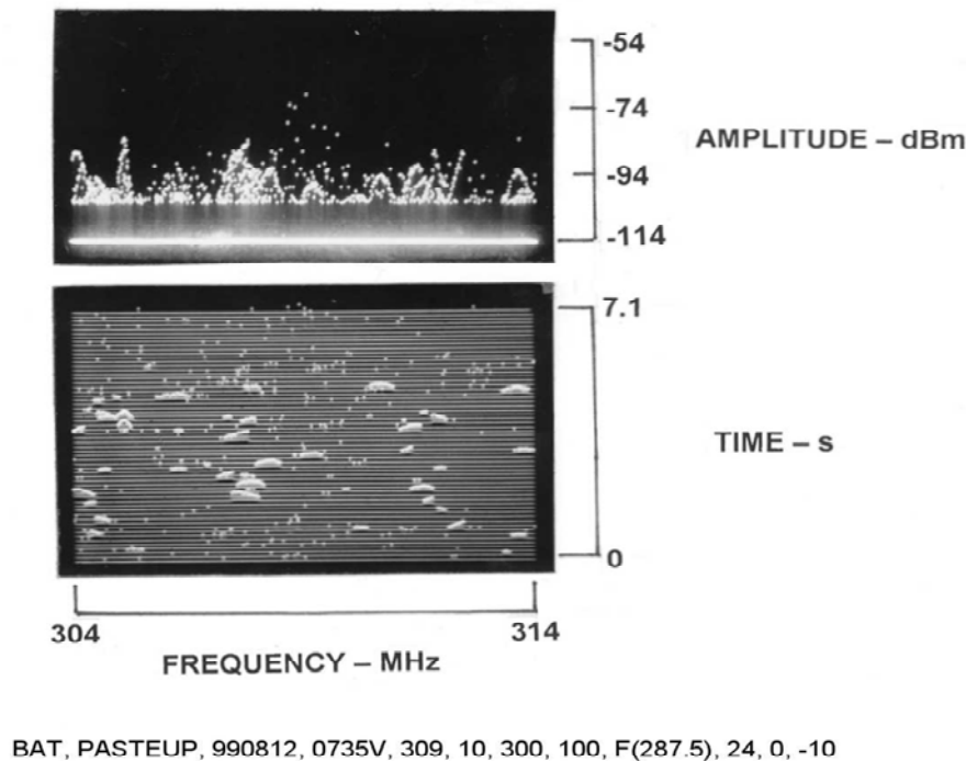
Figure 9 Intermodulation Pulses in the UHF band from a VHF Source
