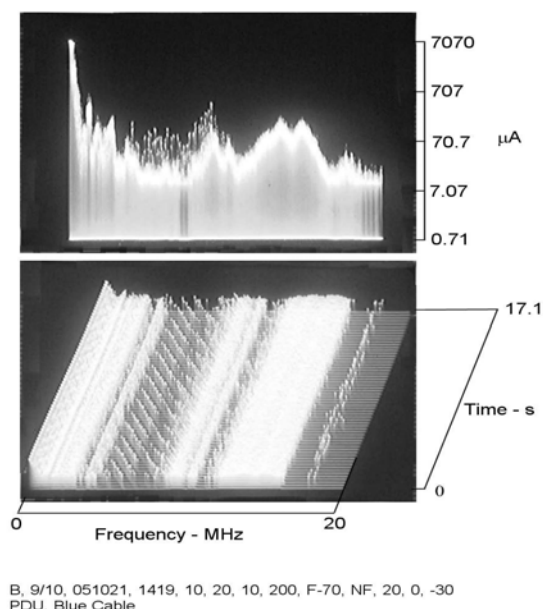
Figure 21 EMI Current Flowing on PDU Power Conductor
