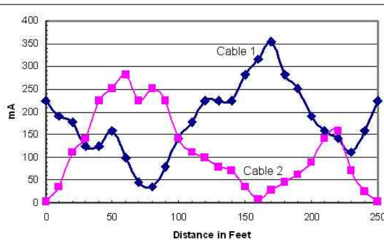
Figure 6 Variation of EMI Current Level on Cable Shields with Distance
